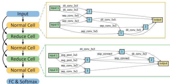
(a) The network architecture searched for the CIFAR10 dataset.
