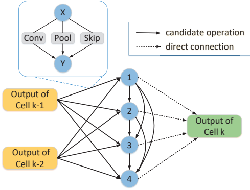
Fig. 2: An example of search space in NAS.
