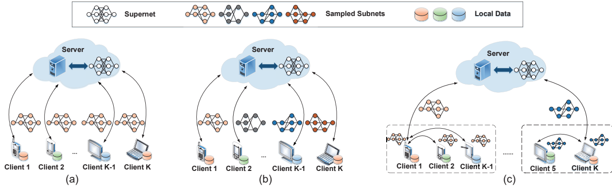
Fig. 1: Illustration of different NAS approaches. (a) OneNAS [17]: the same subnet is allocated to all clients; (b) DecNas [6]: different subnets are allocated to different clients; (c) Our hierarchical NAS: different subnets are allocated to each client cluster and the client in each cluster adopts the same subnet for searching and training.
