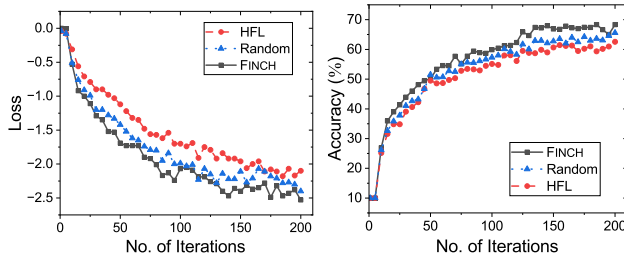
Fig. 6: Loss and test accuracy of three schemes under non-IID setting.
