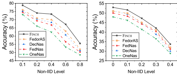
Fig. 8: Test accuracy over the CIFAR10 and ImageNet100 datasets with different non-IID levels.
