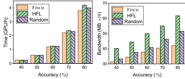
Fig. 7: Resource cost of two schemes with varied target accuracies.
