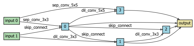
(c) The reduction cell searched for the ImageNet100 dataset.
