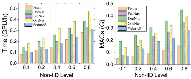
Fig. 9: Resource consumption over the CIFAR10 dataset with different non-IID levels.
