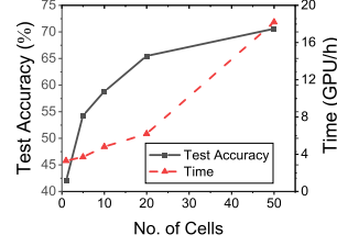
Fig. 3: Test accuracy and completion time with different numbers of cells.
