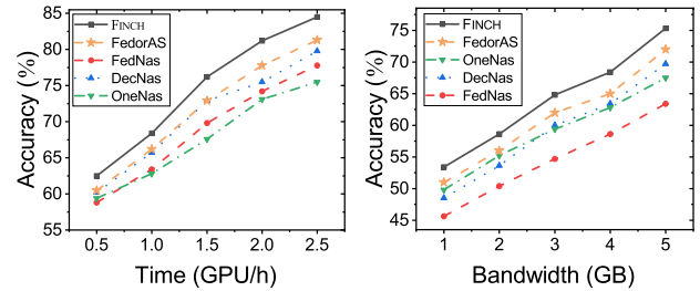
Fig. 10: Test accuracy over the CIFAR10 dataset with completion time and bandwidth constraint.
