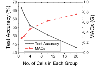
Fig. 4: Test accuracy and completion time with different numbers of cells in each group.
